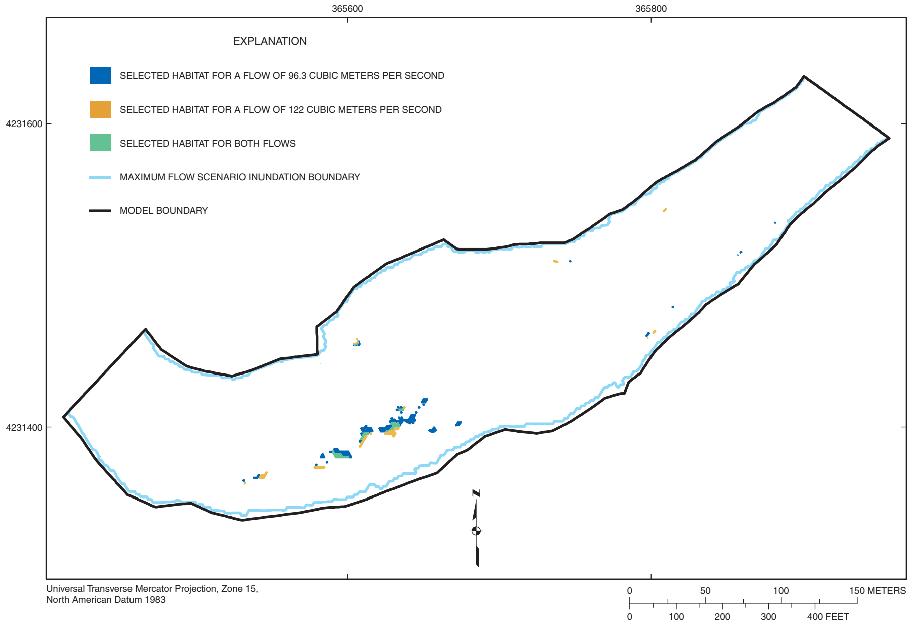
Figure 4-105. Selected habitat area distribution for habitat categories 24, 25 combined (stonecat) at flows of 96.3 and 122 cubic meters per second at Marais des Cygnes River site MDC2.
